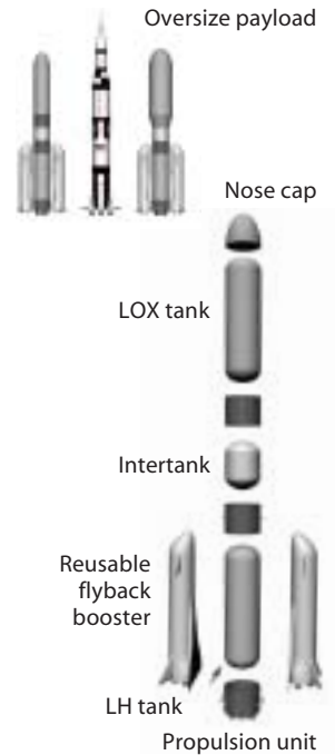
Shuttle-derived heavy space launch system uses a vertically stacked arrangement to provide flexibility in carrying oversize payload and to facilitate reuse of the core propellant tanks in building large orbiting facilities. This configuration uses fully reusable flyback boosters derived from the first stage of the fully reusable TSTO space access systems.
