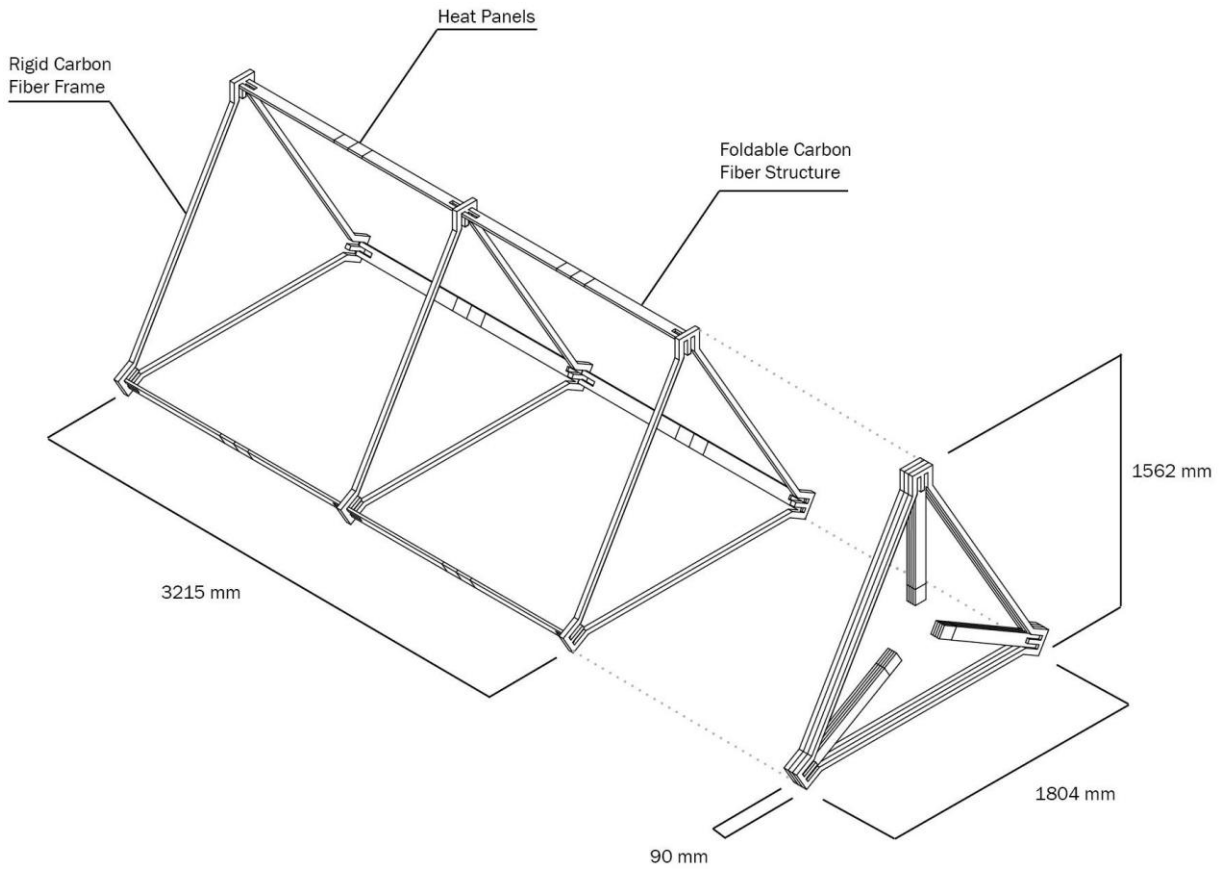
Figure 14: Chosen Truss Design
